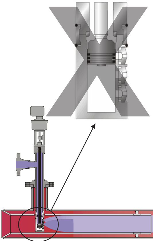
Figure 4: Section view of a conventional attemperator design.
