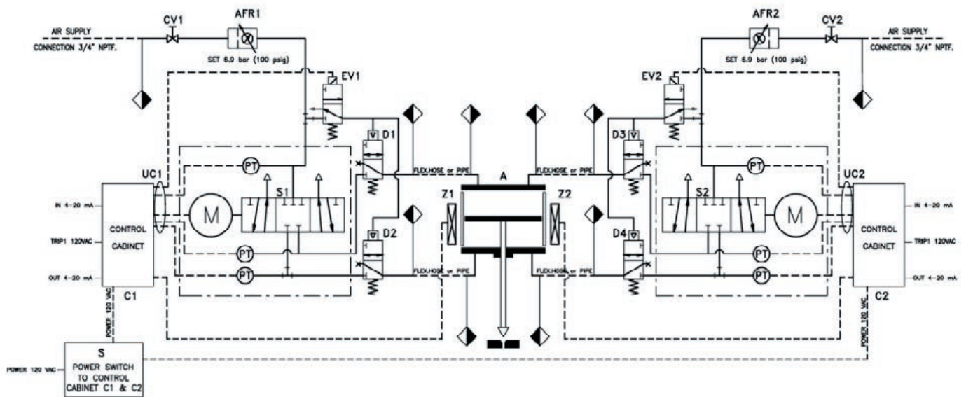
Figure 4: Advanced Smart Positioner
